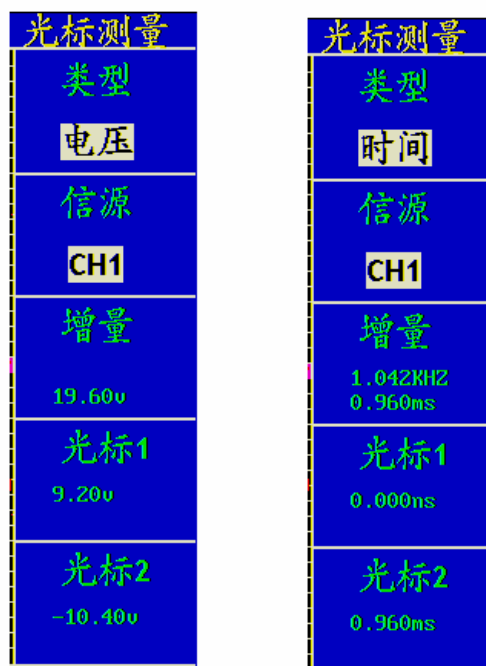
图51：光标测量菜单
