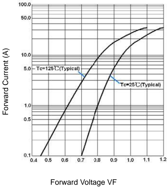
Fig.3 Forward Voltage
