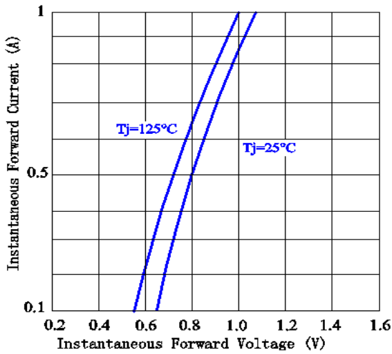
FIG3: Forward Voltage
