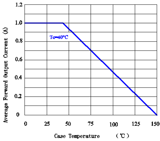
FIG1: I_o - T_c Curve
