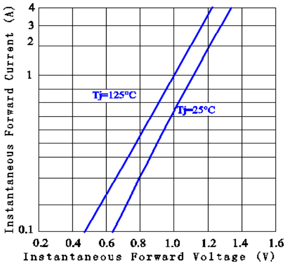
FIG3: Forward Voltage
